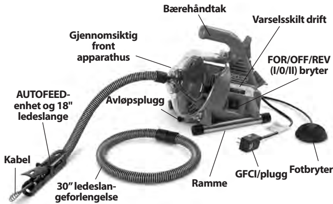
Figur 1 – PowerClear Slukreenser
