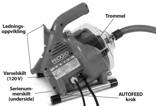
Figur 2 – PowerClear Slukreenser
